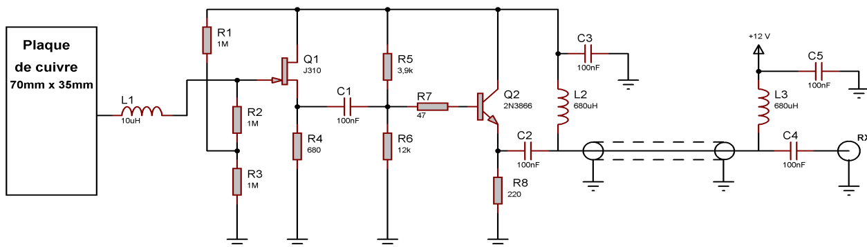
ANTENNE WHIP
