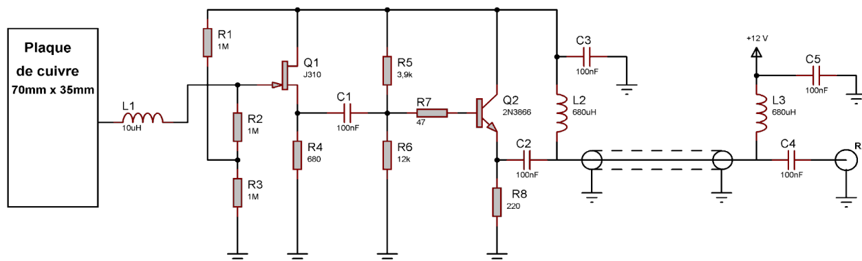
ANTENNE WHIP
