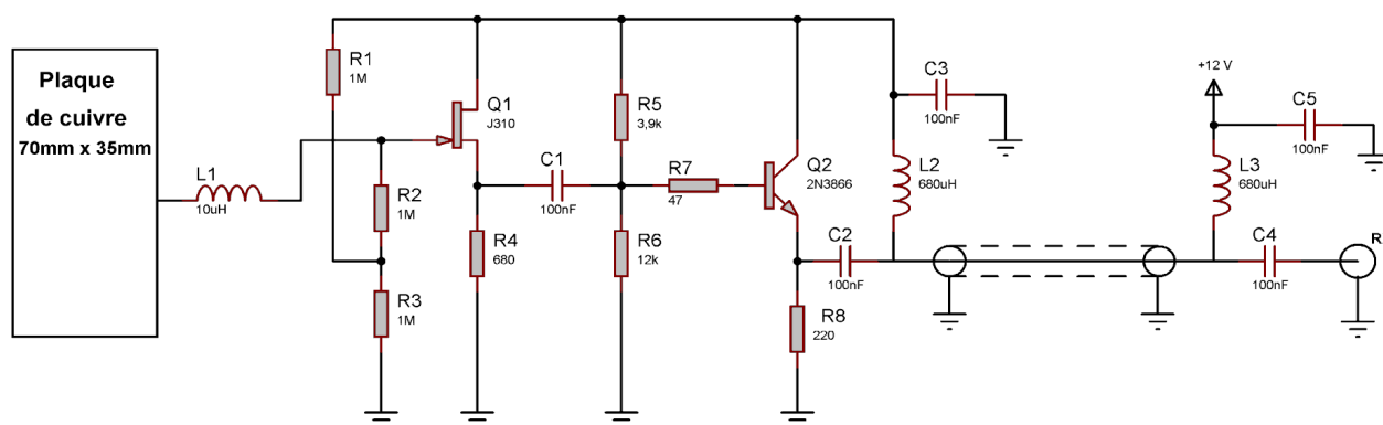
ANTENNE WHIP
